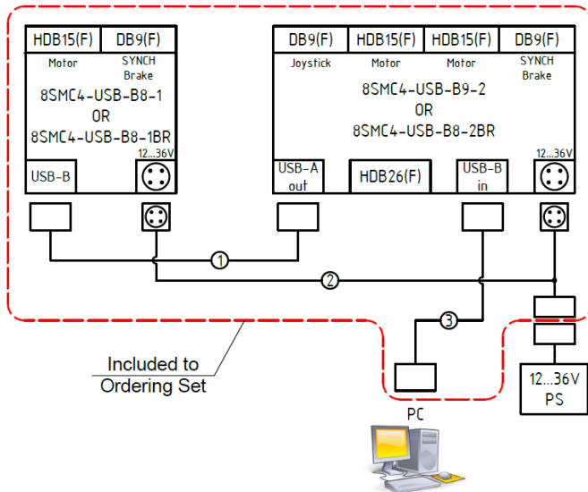
Figure 1. 3-axis controller 8SMC4-USB-B8-B9
